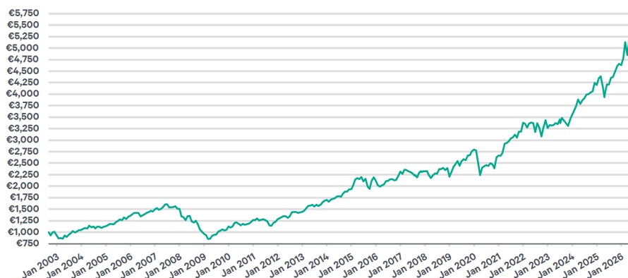
Figure 1: Performance for IQ EQ Global Equity Income Fund as at 30th June 2026
