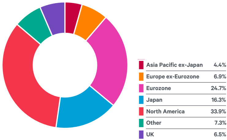
Figure 3: Relative Duration Breakdown (Contribution YRS) 4
